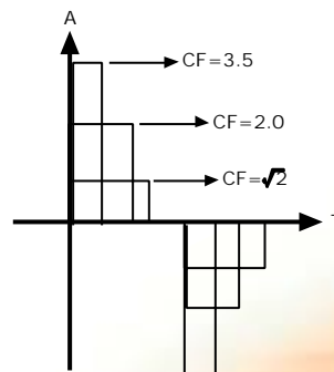
Crest Factor = \sqrt{2} -3.5 Current Waveform of Square-wave
