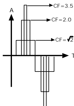
Crest Factor = \sqrt{2} -3.5 Current Waveform of Pulse-wave
