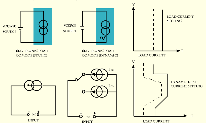
CONSTANT CURRENT MODE APPLICATION
