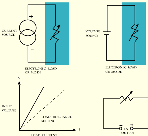
CONSTANT RESISTANCE MODE APPLICATION
